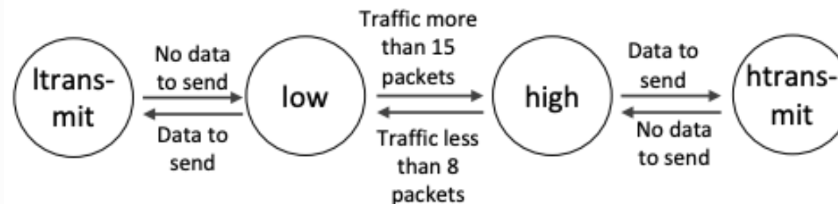
Figure 3: Wi-Fi interface power states.
